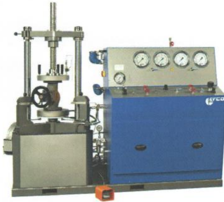
Modular test bench (PS) for testing shut-off and safety valves with air / nitrogen and water
